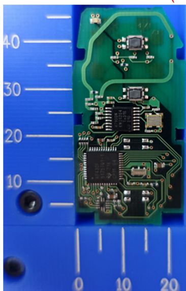
2-Button type
