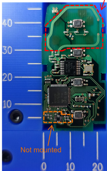
4-Button type
