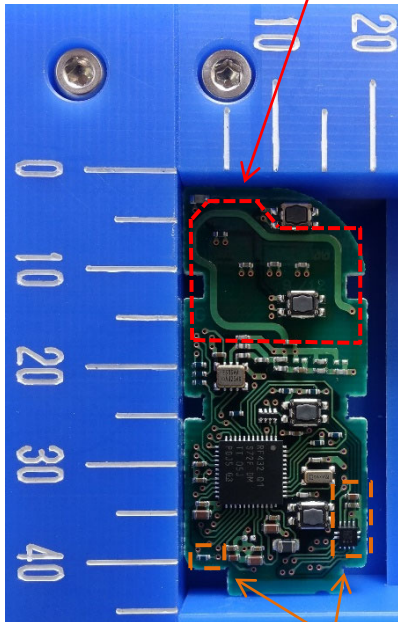
4-Button type IC3, R9, C51, C52
