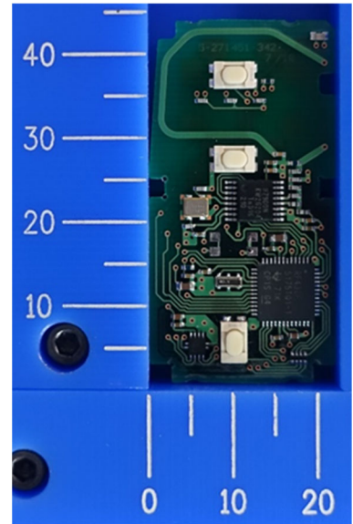
3-Button type
