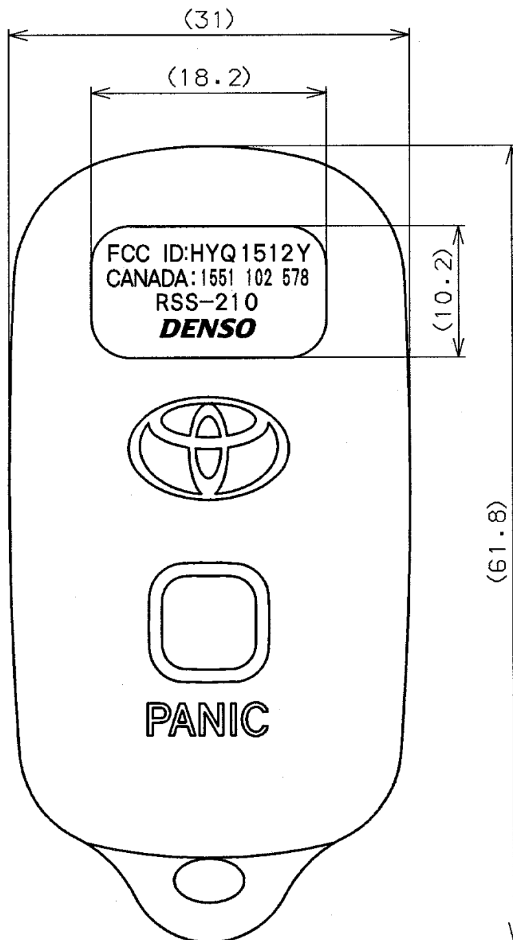
Fig. Marking location and layout of Transmitter
