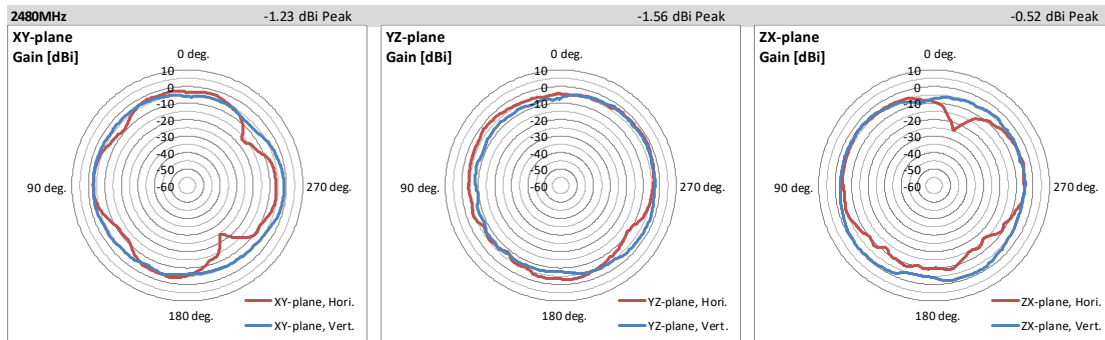
Antenna gain [UNIT: dBi]
