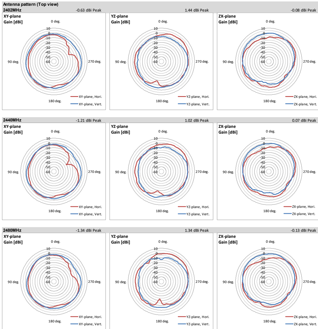
Antenna gain [UNIT: dBi]
