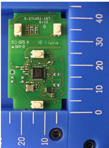
4-Button type
