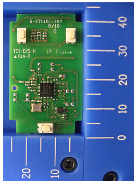
3-Button type
