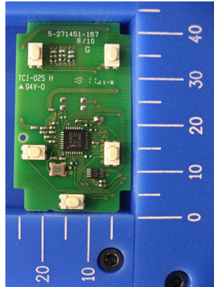
5-Button type
