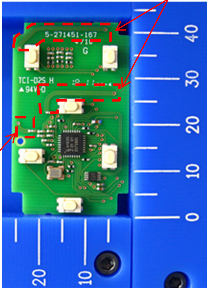
6-Button type
