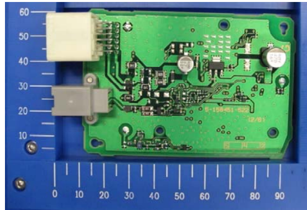
Component Side without antenna
