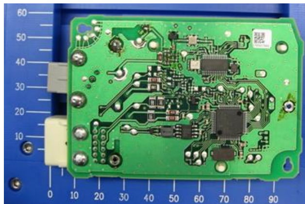
Solder Side
