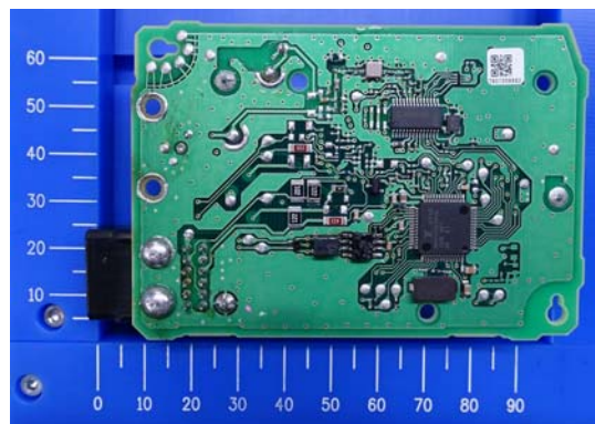
Solder side
