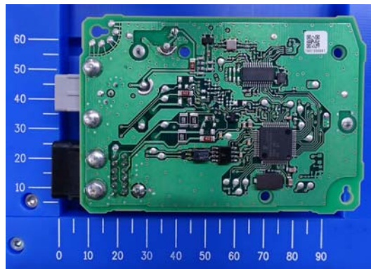
Solder side
