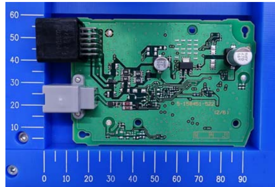
Component side without antenna
