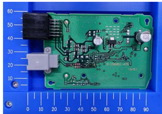
Component side without antenna
