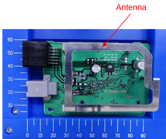
Component side with antenna
