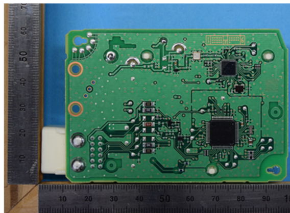
Solder side
