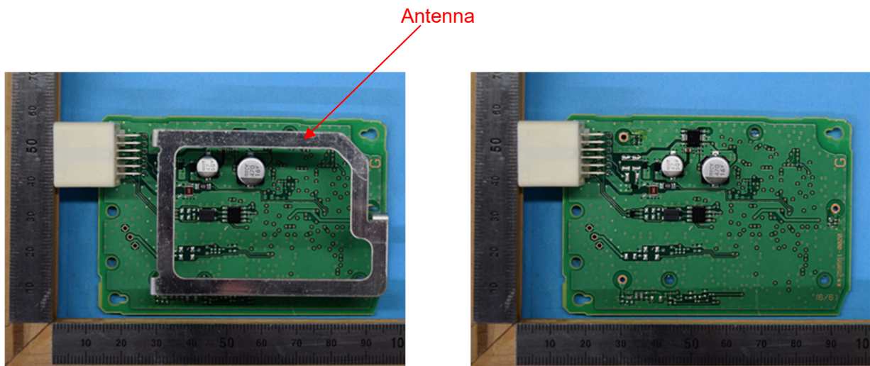
Component side with antenna
