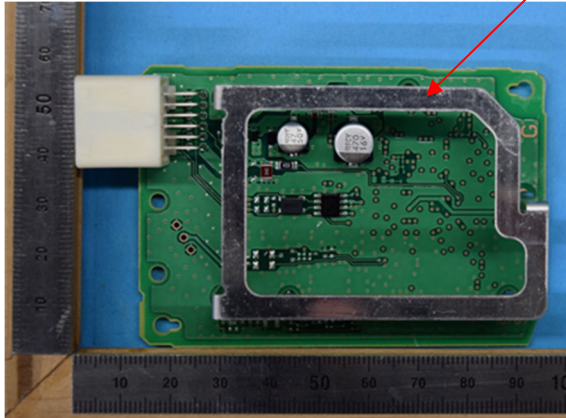
Component side with antenna
