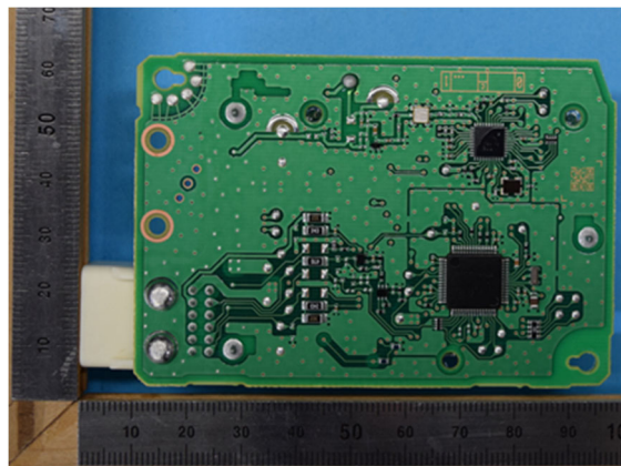
Solder side
