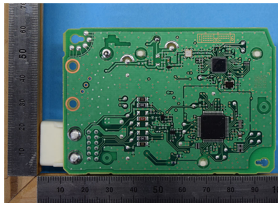
Solder side
