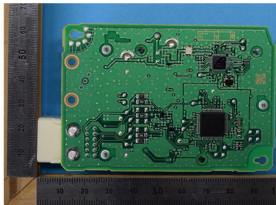
Solder side
