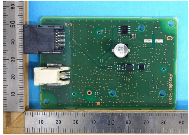
Component side without antenna
