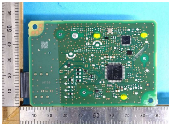
Solder side
