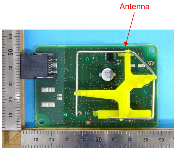
Component side with antenna
