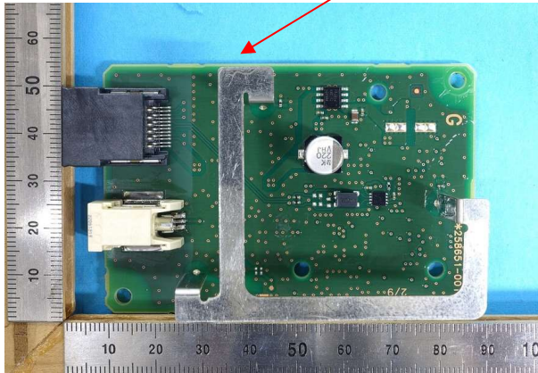
Component side with antenna
