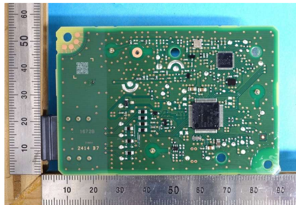
Solder side
