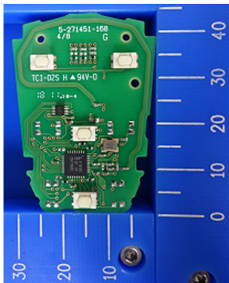
4-Button type
