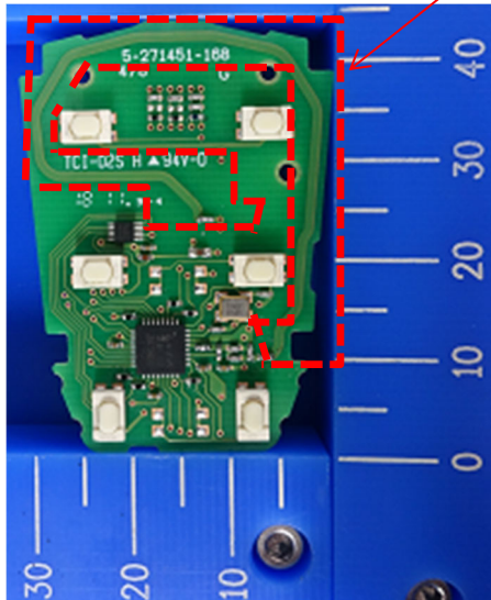
6-Button type
