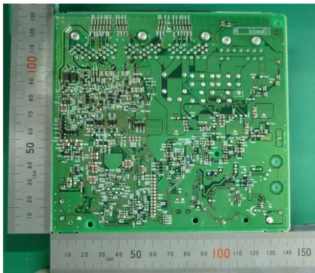
Solder side
