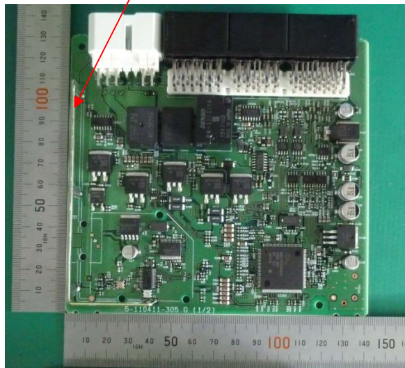
Component side with antenna
