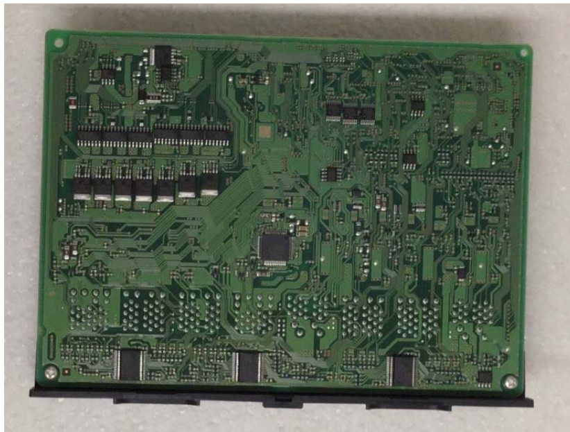
Solder side
