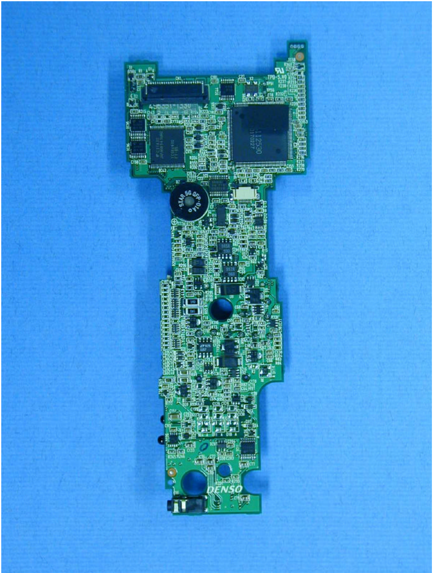
Fig. Component Layout of Main circuit (Component side)
