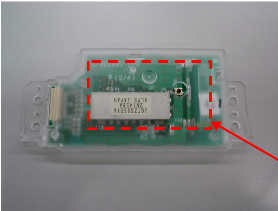
Fig. 4.5.2. Label Location on Bluetooth ASSY
