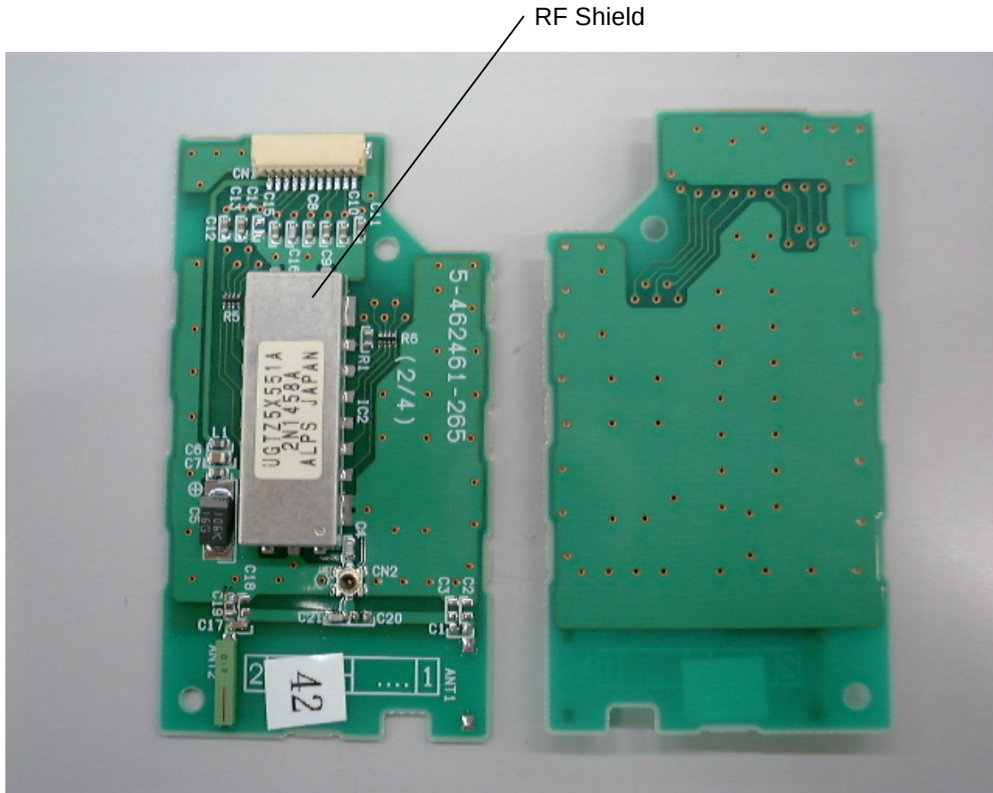
Fig. 4.5.1. Photo of Bluetooth ASSY PCB Layout
