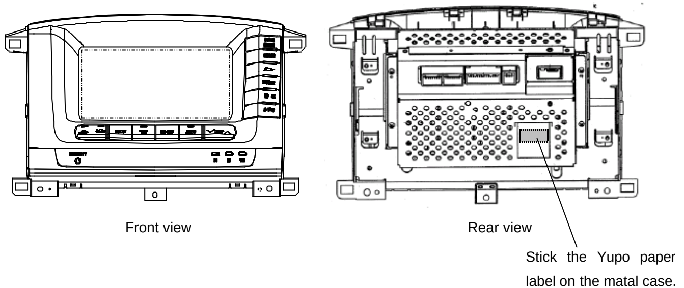
Fig. 4.6.1. FCC and IC Label Location on Navigation ASSY
