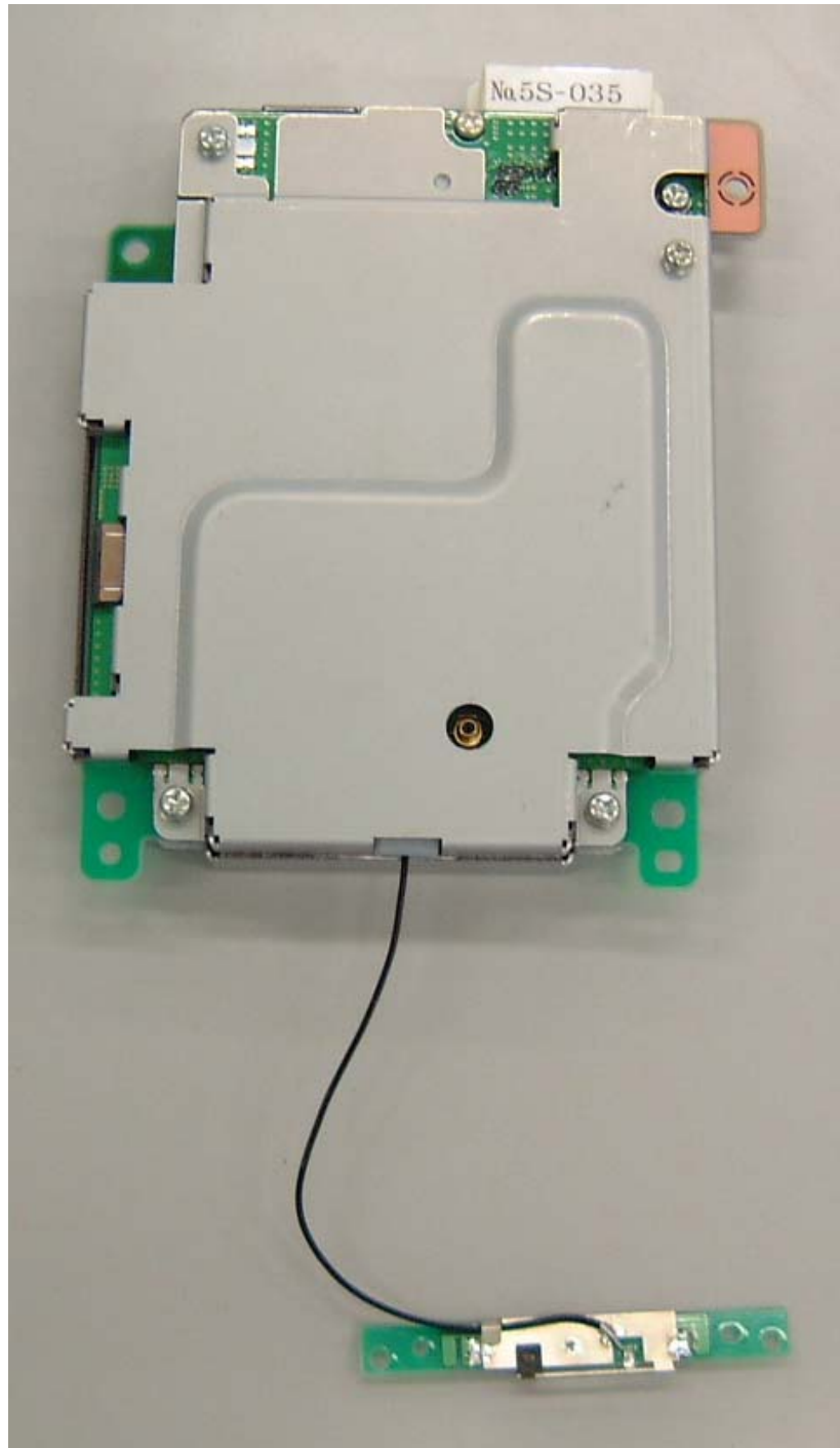
Audio Bluetooth Hands Free Unit (BTAU02A)
