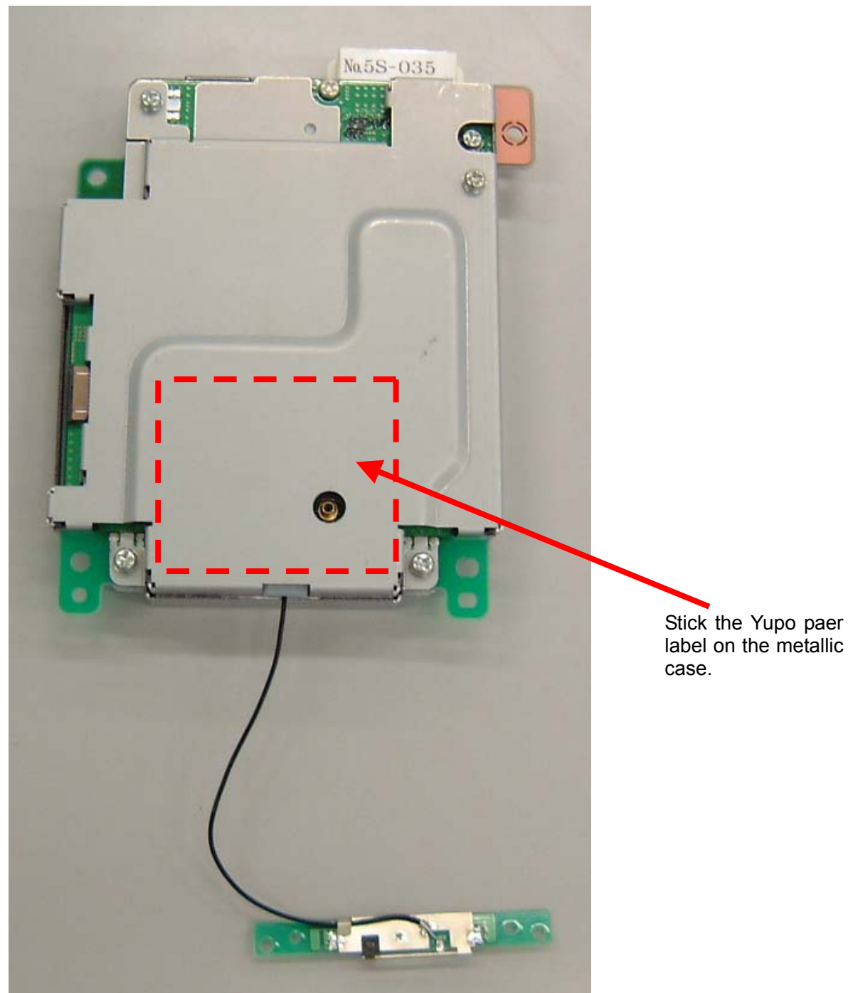
Fig. 4.5.1b. Label Location on Audio Bluetooth Hands Free Unit (BTAU02A)
