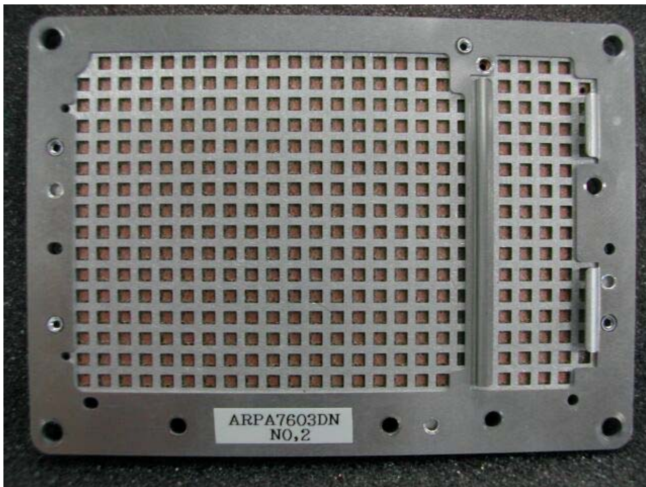
EUT inside view antenna section front side
