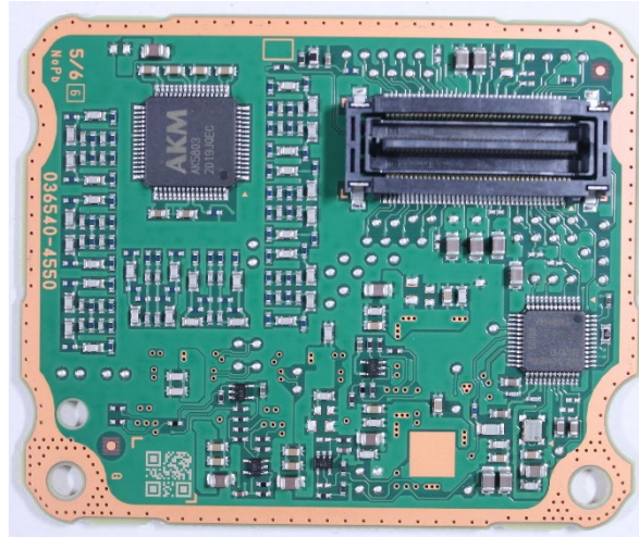
Component side
