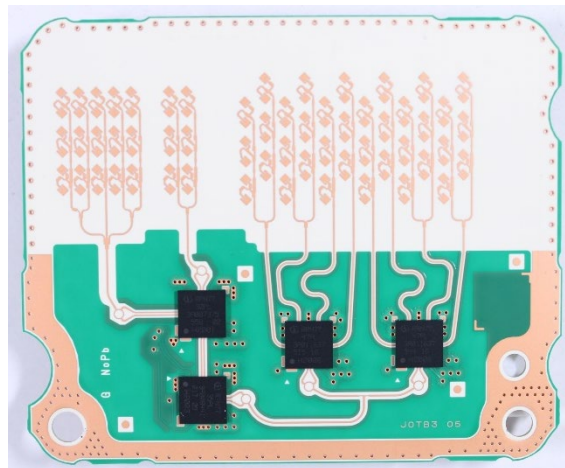
Antenna side
