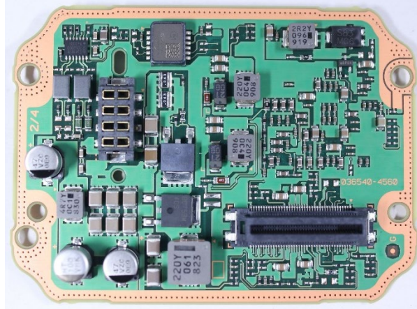
Component side A
