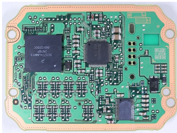
Component side B
