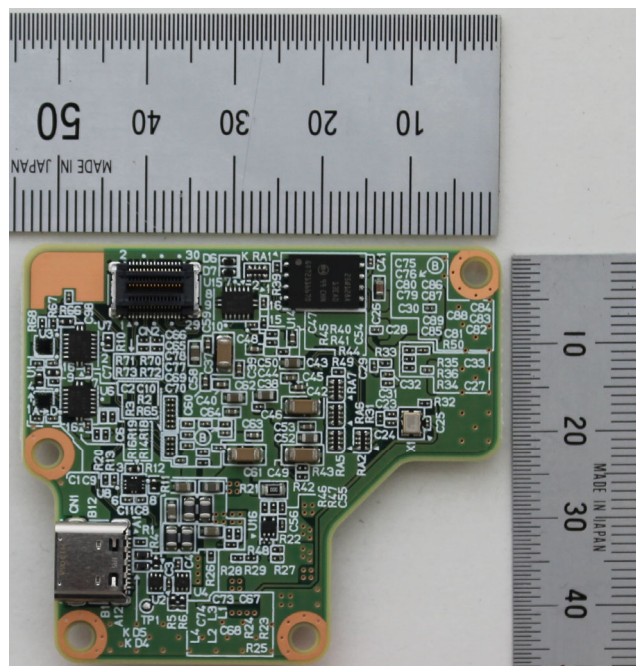
Component side B
