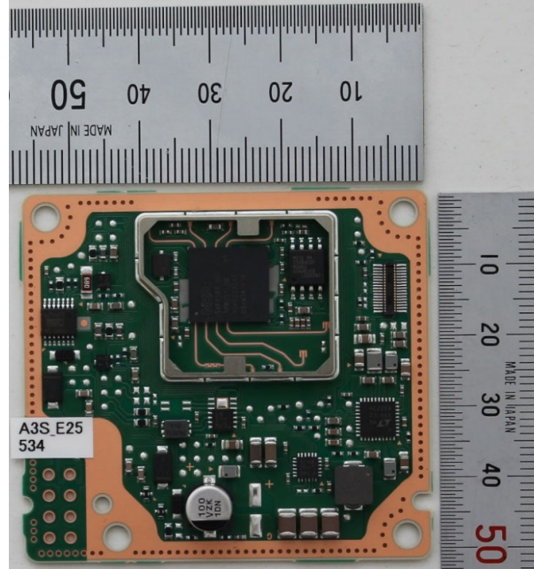
Component side (Without shield)
