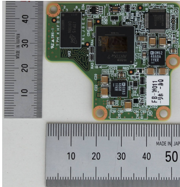
Component side A
