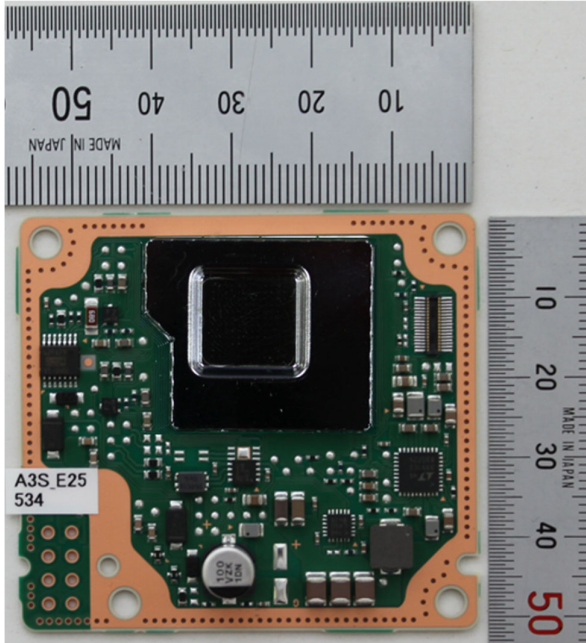
Component side (With shield)
