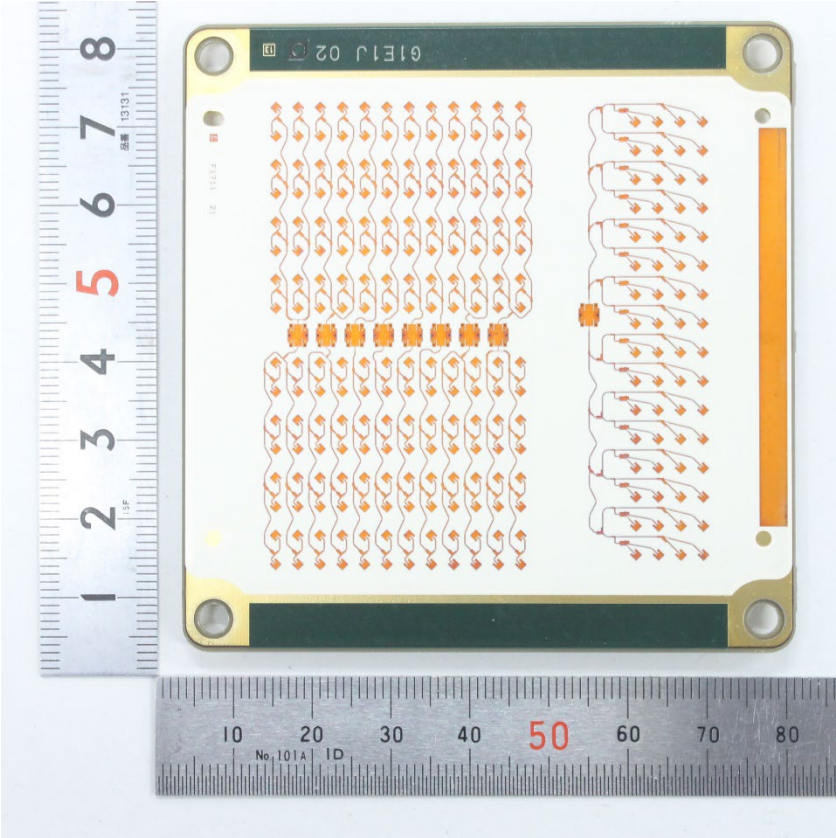
Antenna side
