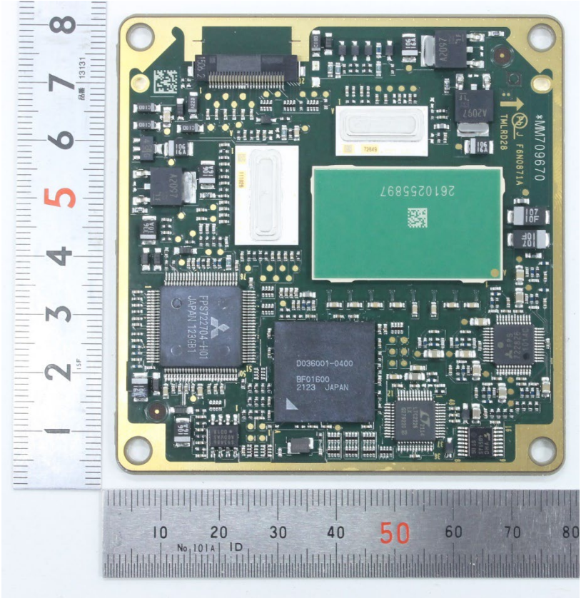
Component side
