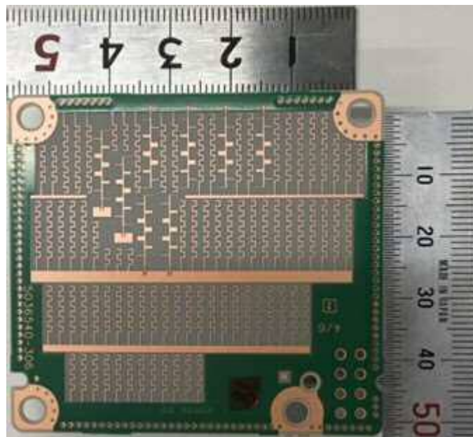
Antenna side
