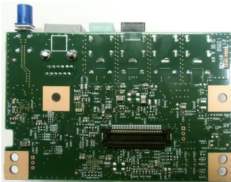
Solder Side
