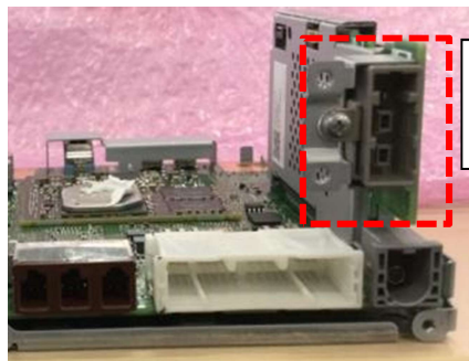
Radio Tuner Connector
