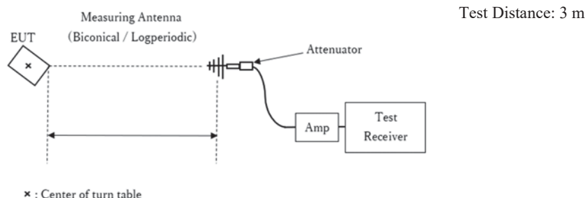
Figure 2: Test Setup
