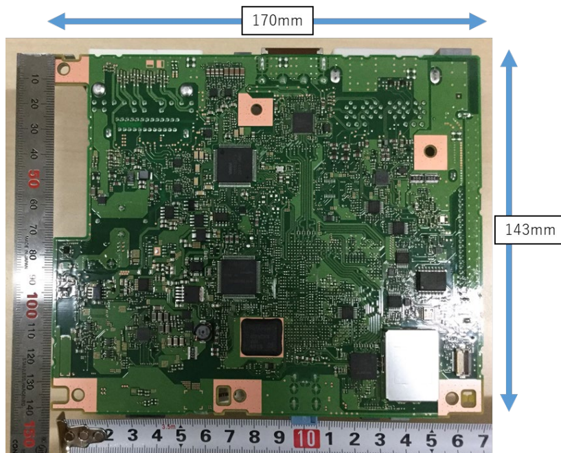
Component Side(Cockpit Control Unit) – Main PCB
