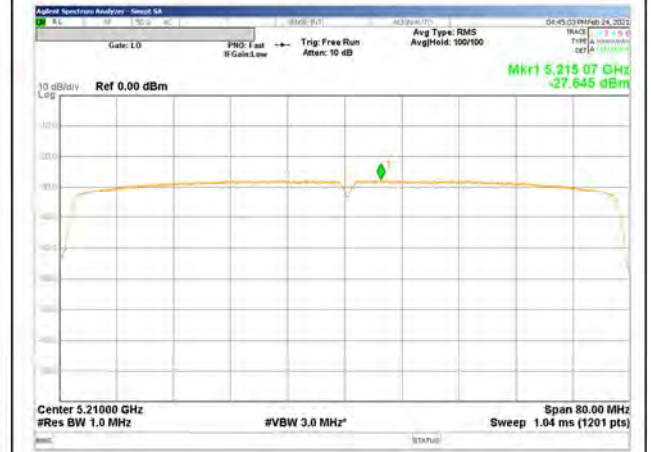
11ac-80 MIMO, Chain 1
