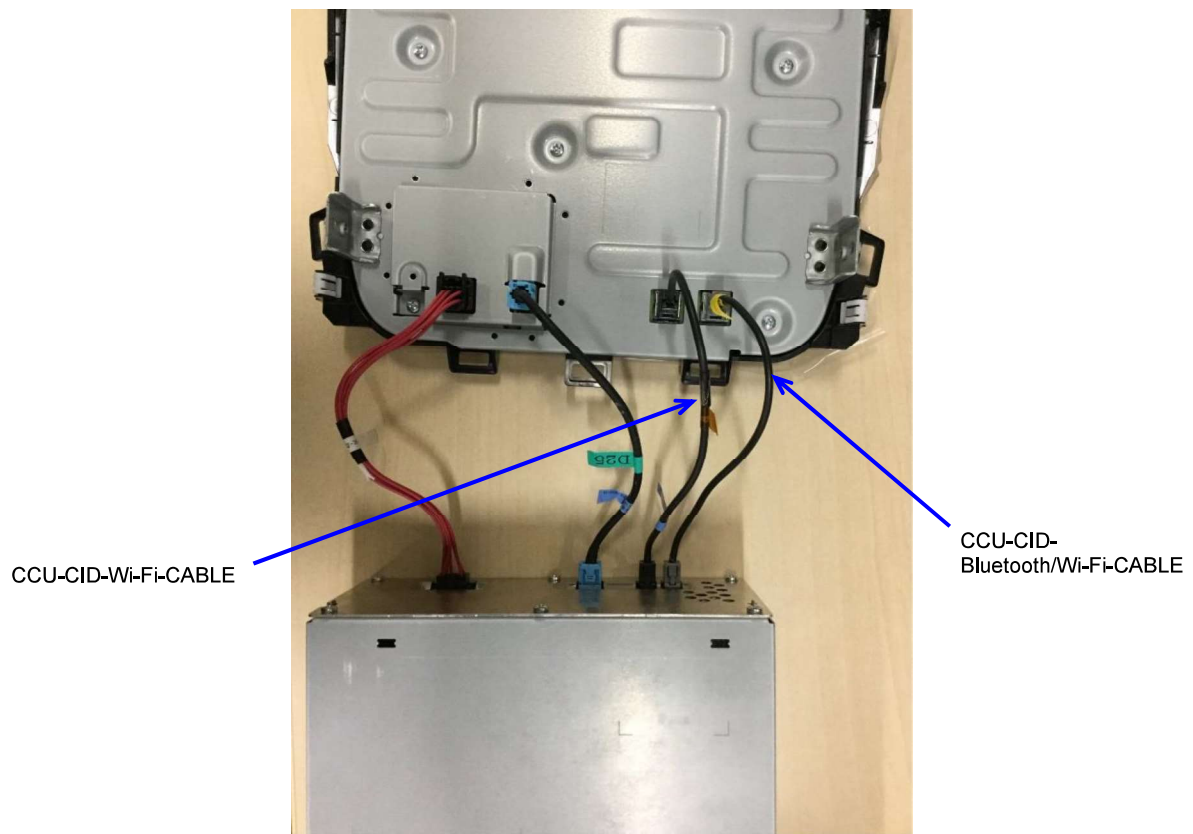
Connection part of the CCU and CID
