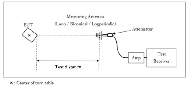
Figure 1: Test Setup
