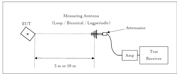
Figure 2: Test Setup Below 1 GHz
