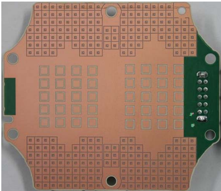
Antenna side
