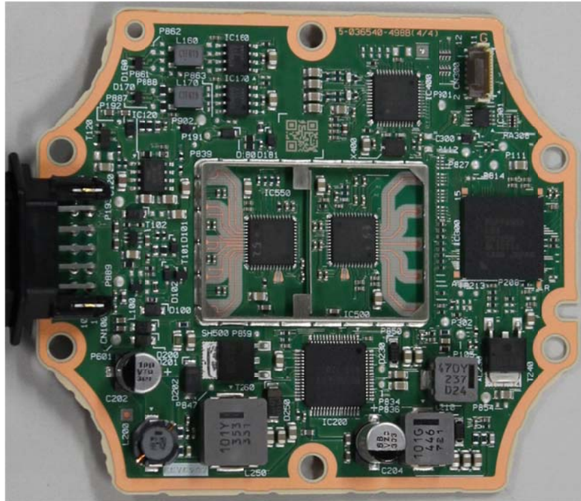
Component side
