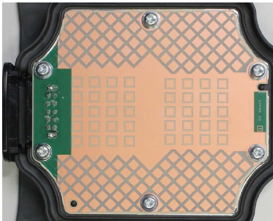
Antenna side
