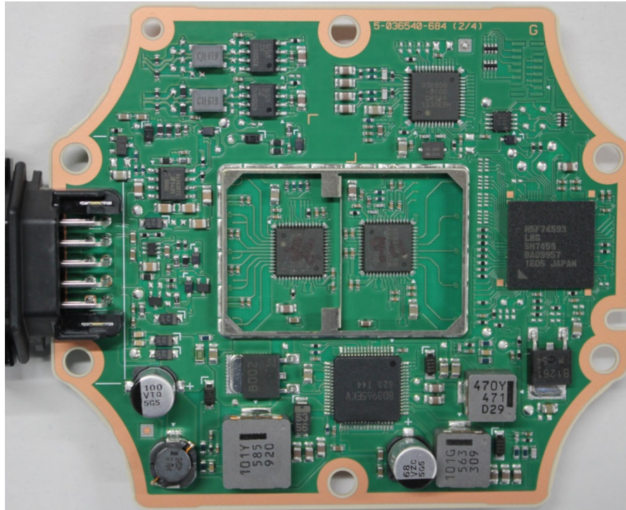
Component side
