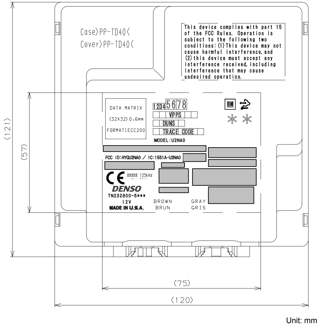
Fig. Marking location and layout of UPE
