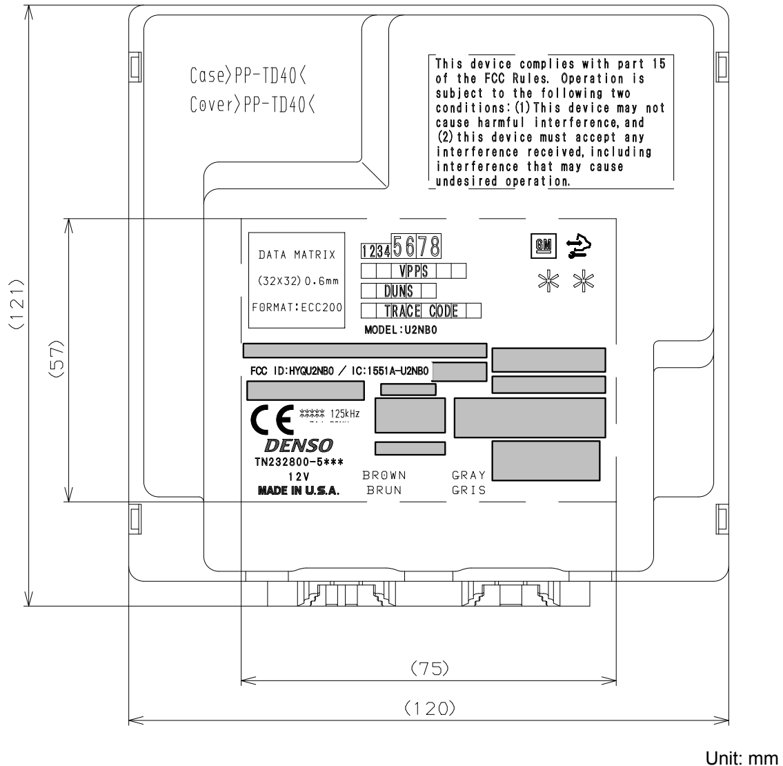
Fig. Marking location and layout of UPE
