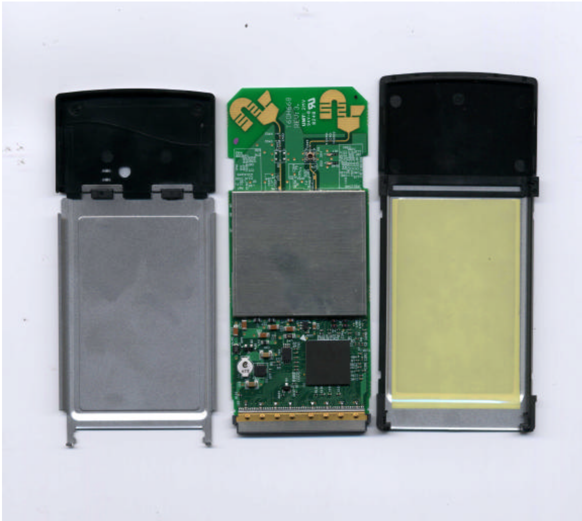
Inside View of Covers and PCB:
