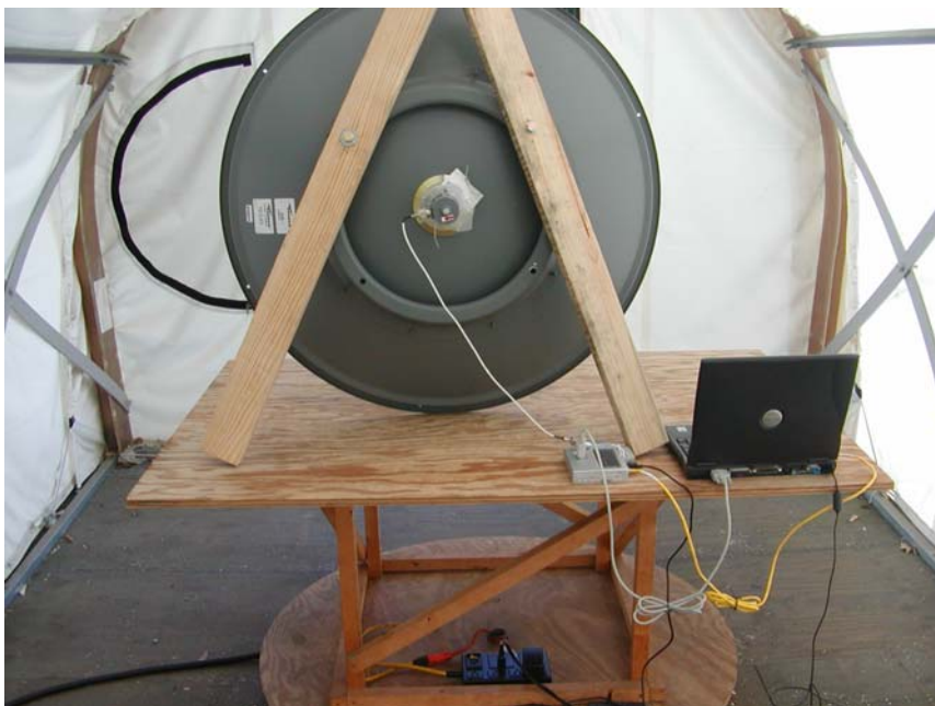
Radiated Emission with P3F-52-N7A Dish Antenna - Rear View
