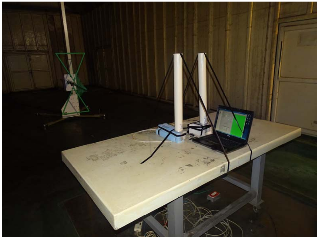
Back View of Radiated Test-Omni
