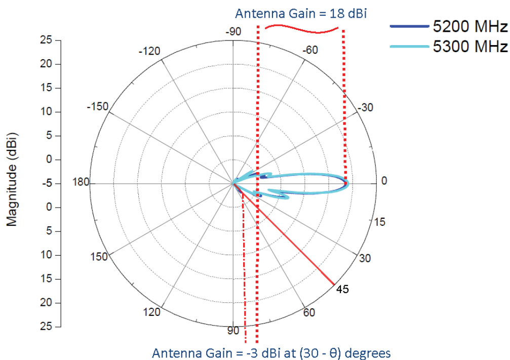
Figure 8-6 Antenna gain at (30 - \theta) = 45^\circ
