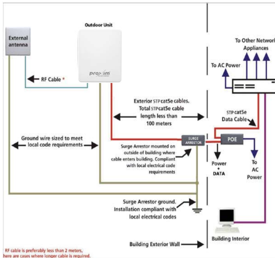
Figure 8-7 Cable Setup
