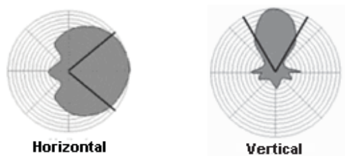
Figure 7-2 Sector Antenna Coverage
