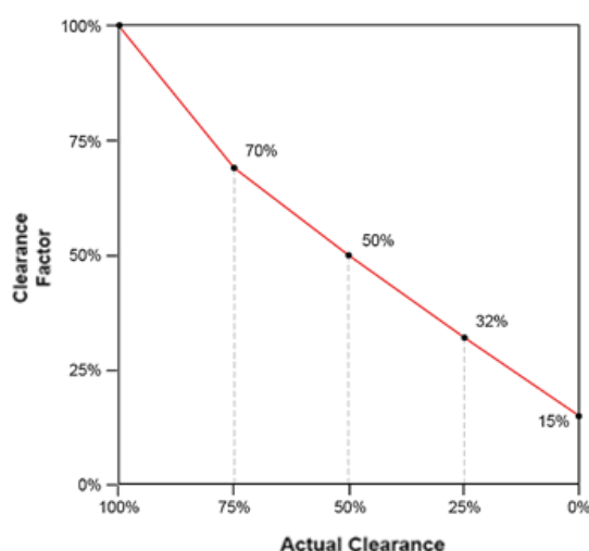
Figure 9-3 Clearance Factor
