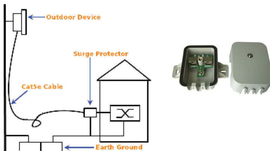
Figure 4-6 Surge Protector
