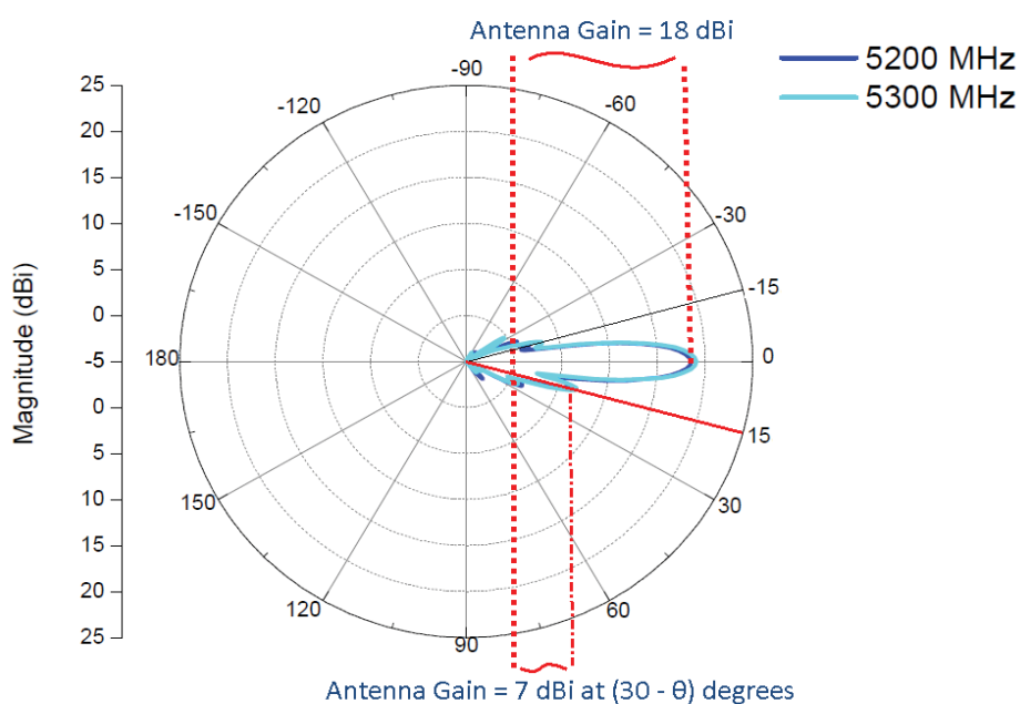
Figure 8-5 Antenna gain at (30 - \theta) = 15^\circ
