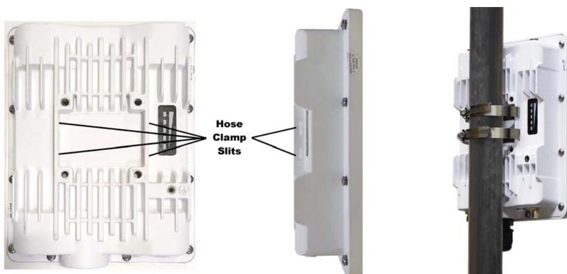
Figure 4-4 Pole Mounting (Edge 1035, 1045 and 1055)
