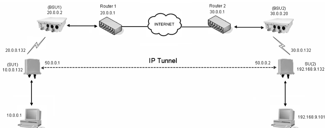
Figure 5-19 An Example: Tunnel Configuration
