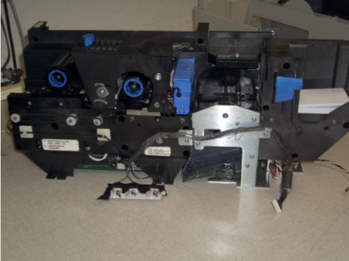
EUT front & cover removed
