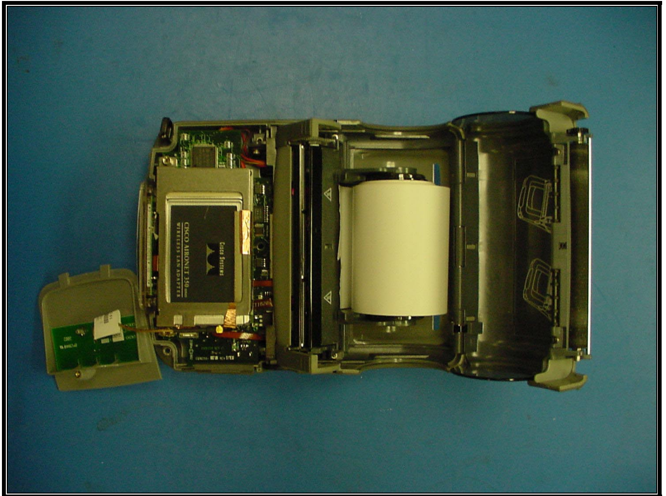
PHOTOGRAPH 13: INSIDE PRINTER
