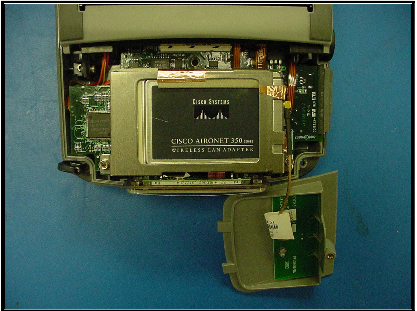
PHOTOGRAPH 14: WLAN ADAPTER AND ANTENNA
