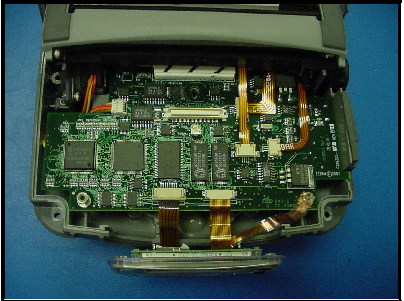
PHOTOGRAPH 12: INSIDE PCB
