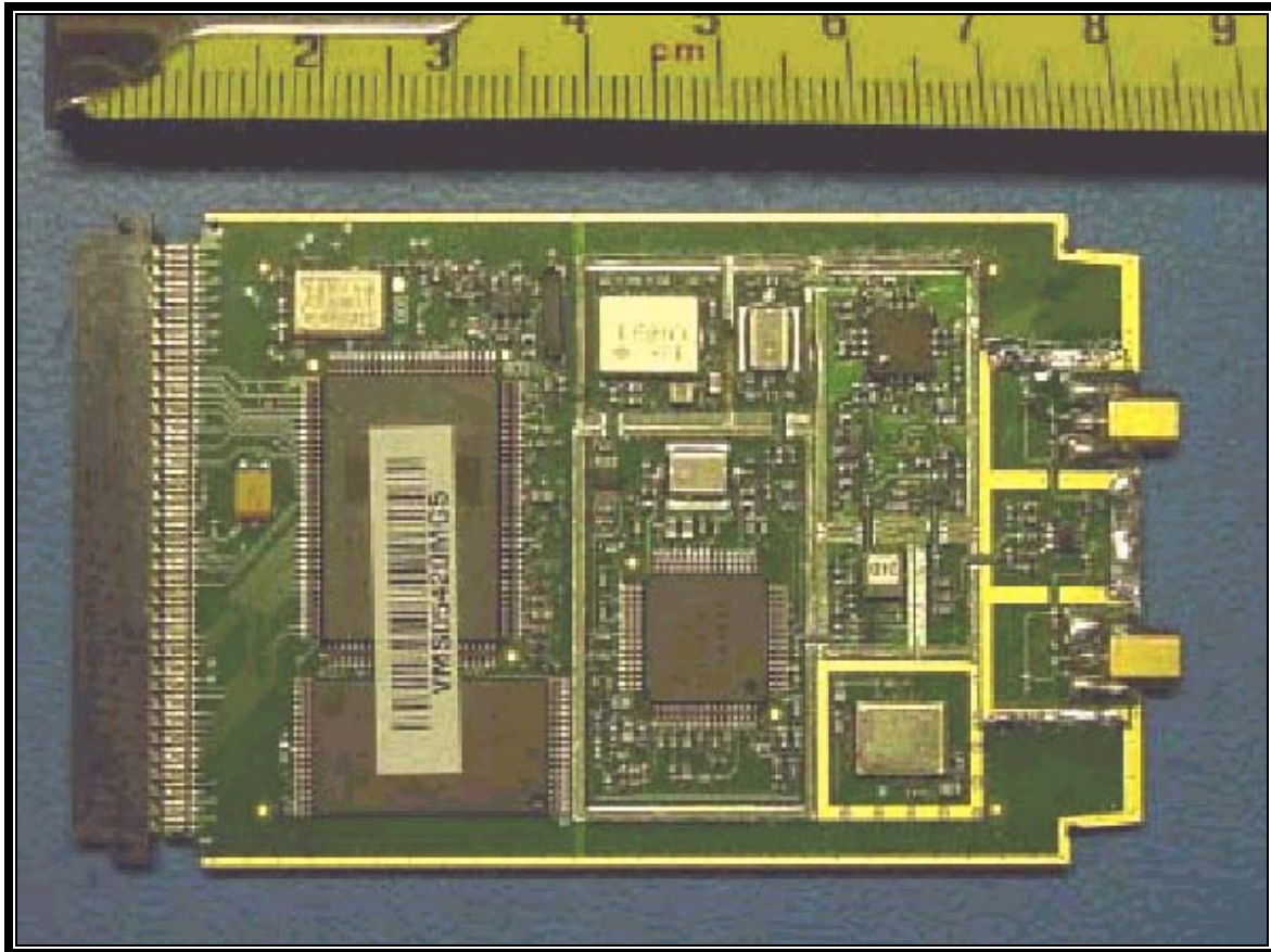
PHOTOGRAPH 23: WLAN BACK VIEW OF PCB WITHOUT SHIELDS
