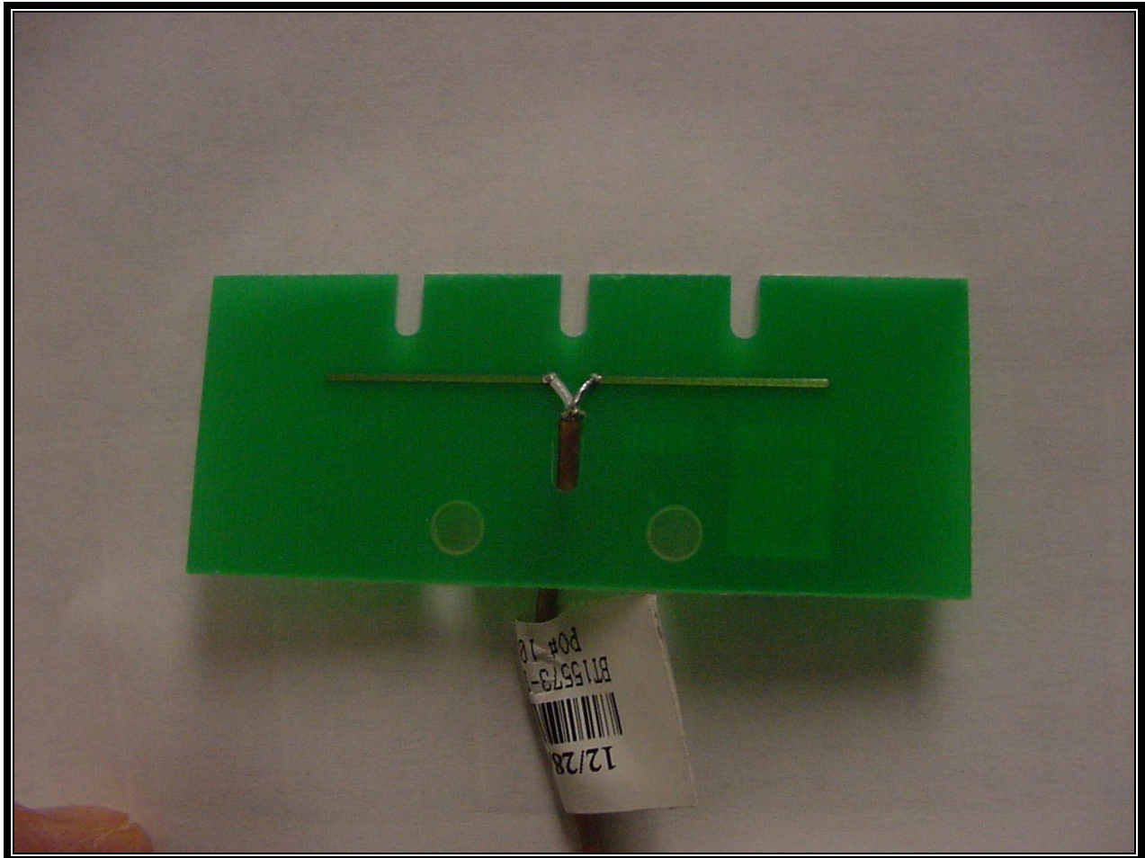
PHOTOGRAPH 15: ANTENNA TOP VIEW
