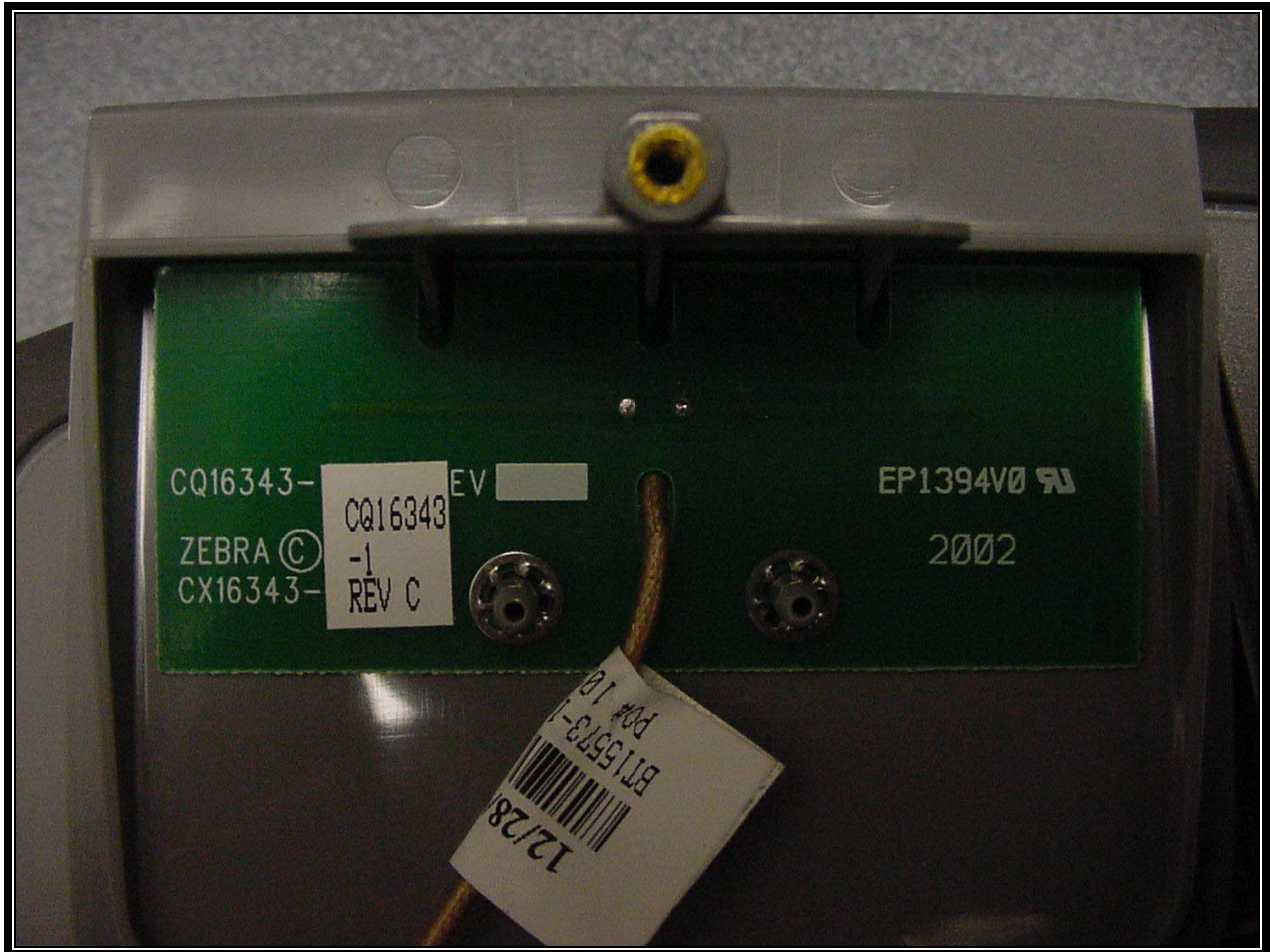
PHOTOGRAPH 17: ANTENNA CONNECTED TO COVER
