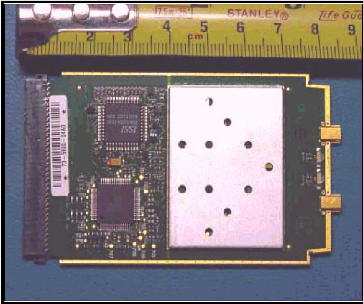
PHOTOGRAPH 20: WLAN ADAPTER FRONT VIEW OF PCB WITH SHIELD
