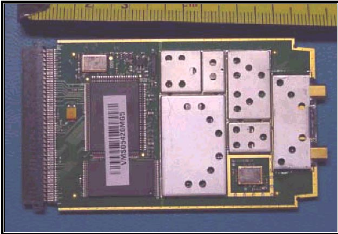
PHOTOGRAPH 21: WLAN BACK VIEW OF PCB WITH SHIELDS
