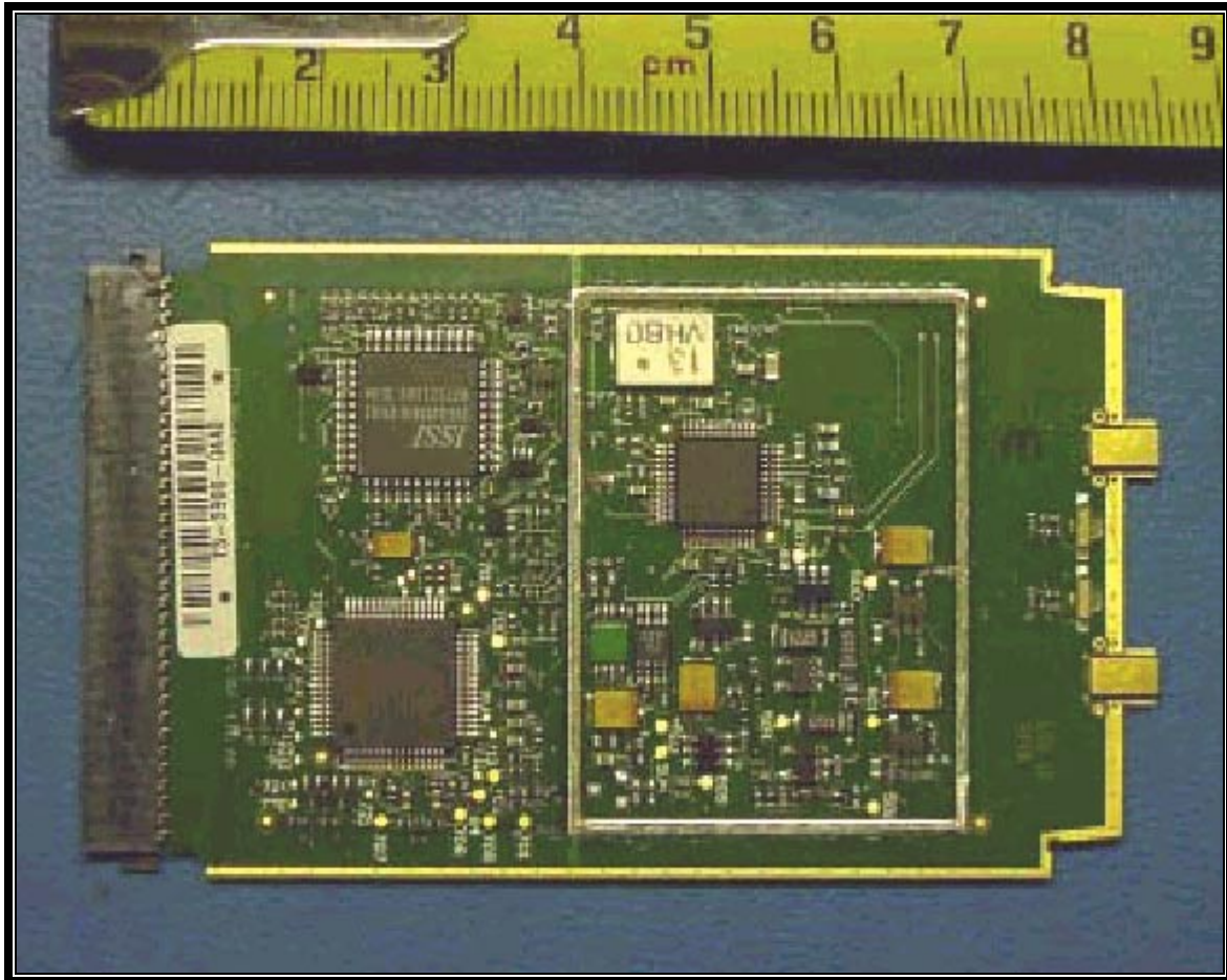
PHOTOGRAPH 22: WLAN FRONT VIEW OF PCB WITHOUT SHIELD
