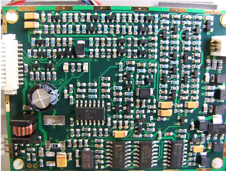
RFID board
