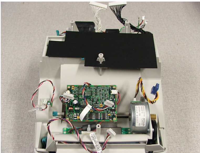
Without PCB board
