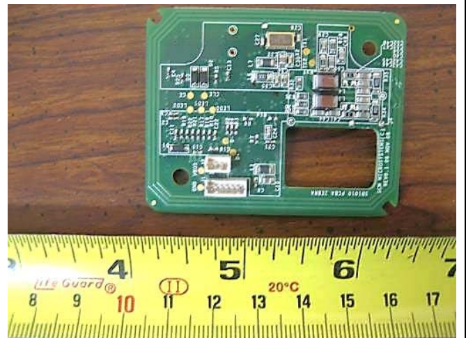
PCBA6 without Shielding Bottom View 1
