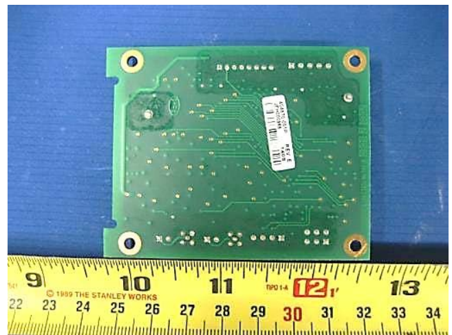
RFID Radio Bottom View
