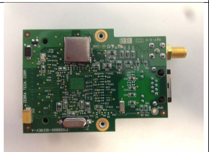
WLAN Radio Board Bottom View
