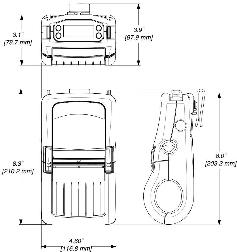
FIGURE 18 OVERALL DIMENSIONS
