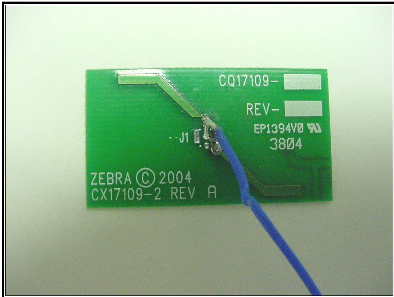
PHOTOGRAPH 49: RW-420 (CQ17109-1) ANTENNA FRONT VIEW
