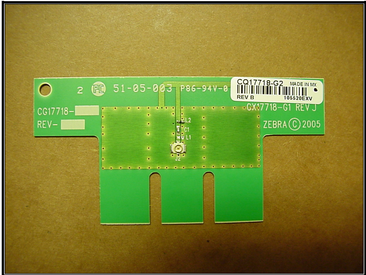
Photograph 11: CQ17718-G2 Antenna Front
