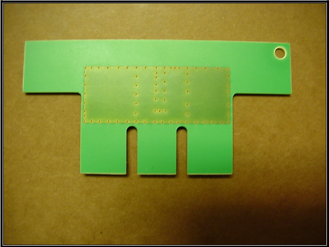
Photograph 10: CQ17718-G1 Antenna Back
