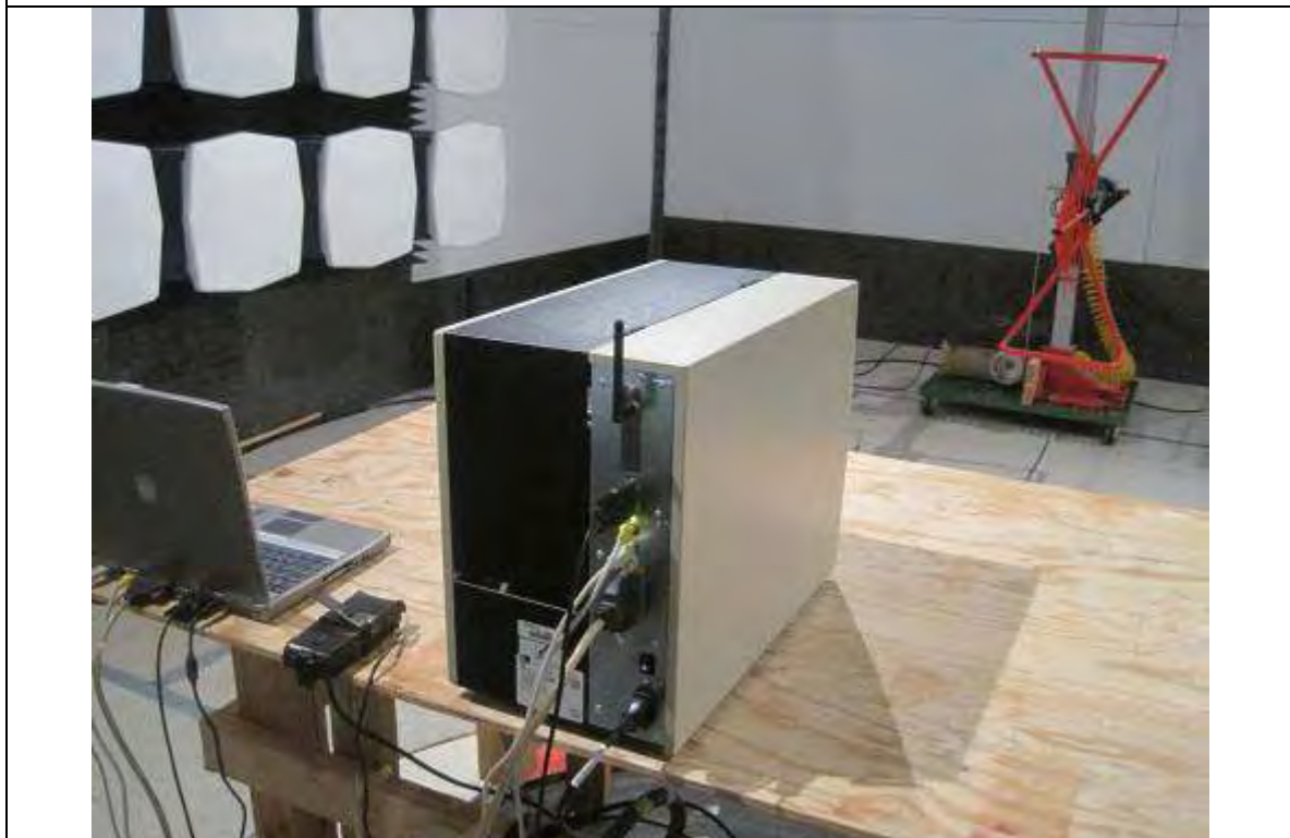
Radiated Emission Test Setup (above 1GHz) – Rear View
