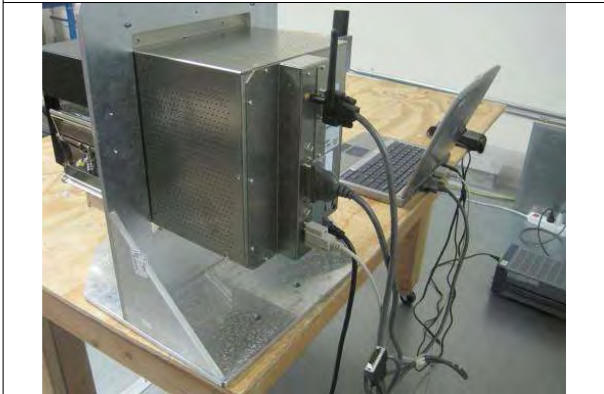
Conducted Emission Test Setup – Rear View
