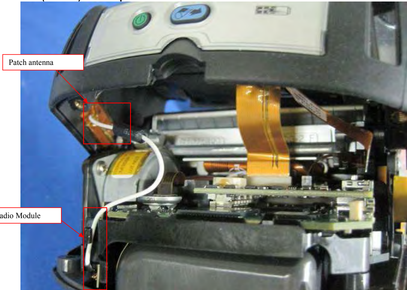
QLn320 Internal View
