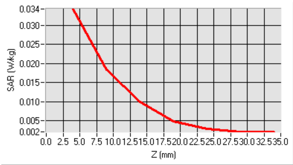
SAR, Z Axis Scan (X = 1, Y = -58)
