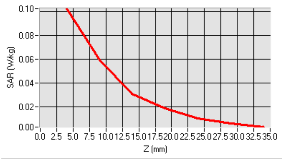
SAR, Z Axis Scan (X = 3, Y = -58)
