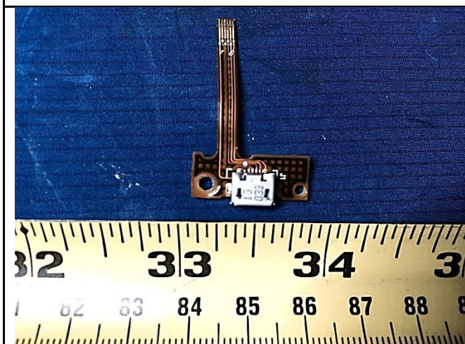
PCBA 5 Top View
